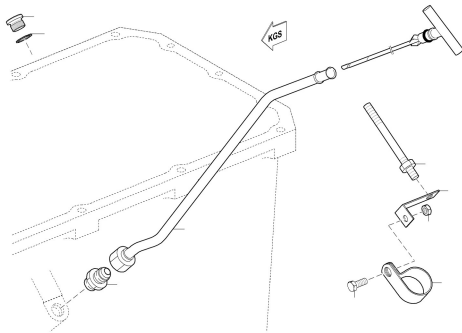
OIL FILLER NECK UPC.06G04 1447
